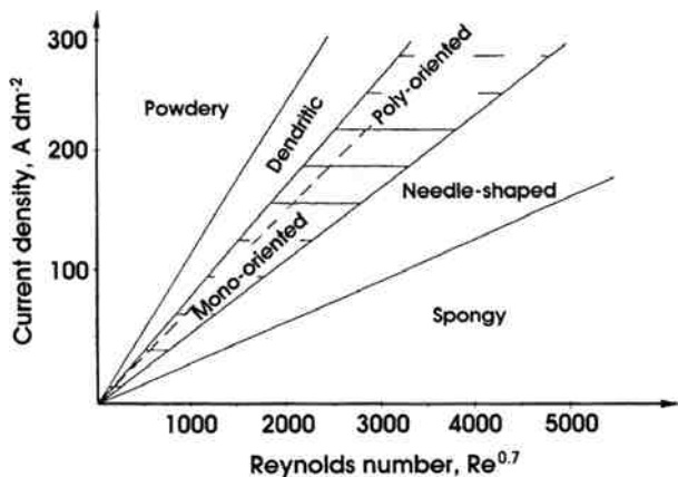
Figure 8 - Morphology diagram for acid zinc in terms of current density and Reynolds number (after Azzeri, et al. ).
