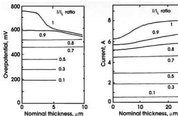
Figure 11 - Electrodeposition at fractions of the limiting current for acid copper sulfate solutions, using the RCE: (a) overpotential/nominal thickness at 900 rpm; (b) current/nominal thickness at 300 rpm (after Robinson and Gabe).
