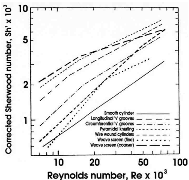
Figure 3 - Enhancement by roughness: Mass transfer correlations ( Sh/Re ) for several types of roughness on a RCE, using acid copper deposition (after Makanjuola and Gabe).
