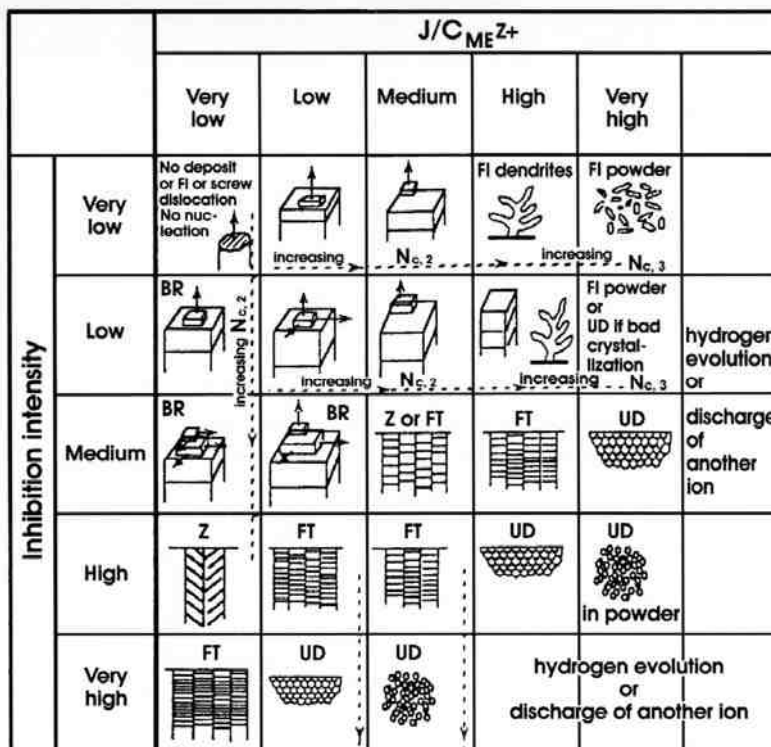
Figure 12 - Morphology diagram showing different types of polycrystalline electrodeposits (after Winand).
