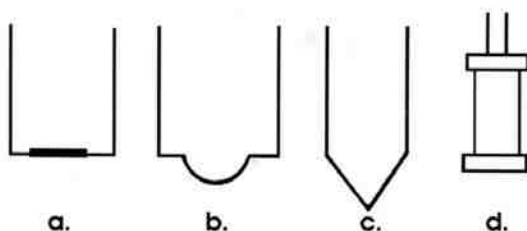
Figure 1 - Types of rotating electrode.
