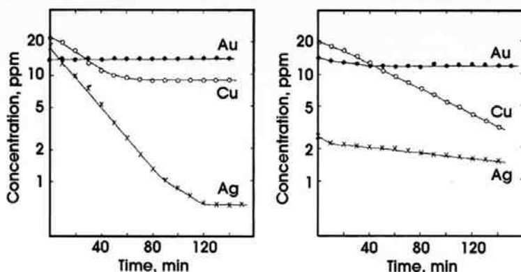
Figure 4 - Potentiostatic separation with the RCE (after Walsh and Gabe).
