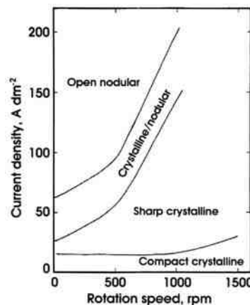
Figure 9 - Morphology diagram for zinc-nickel electrodeposits produced from an acid solution (after Wilcox and Gabe).
