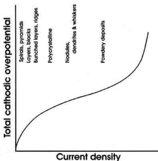
Figure 6 - Cathodic polarization diagram showing ranges of characteristic growth modes.
