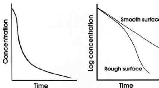
Figure 2 - Concentration-time relationships: (a) exponential decay in batch operation; (b) logarithmic graph for smooth and rough surfaces.
