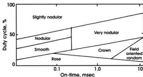
Figure 10 - Morphology diagram of on-time/duty cycle at 6 A/cm 2 and 55°C for pulsed jet (Re = 12,000) plated gold contact spots (after Bocking).
