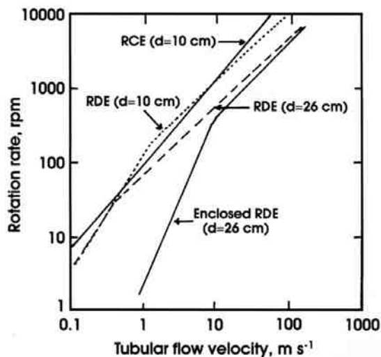
Figure 5 - Graph of RCE and RDE rotation rate against tubular flow velocity, demonstrating flow equivalence in the turbulent regime for a corrosion process (after Heitz).
