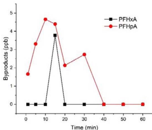
Figure 3 - Shorter chain PFAAs detected during the electrooxidation of PFOA in 100 mM Na 2 SO 4 solution with TSO anode. Initial concentration = 2.0 μM (828 ppb for PFOA), current density = 5.0 mA/cm 2 .
