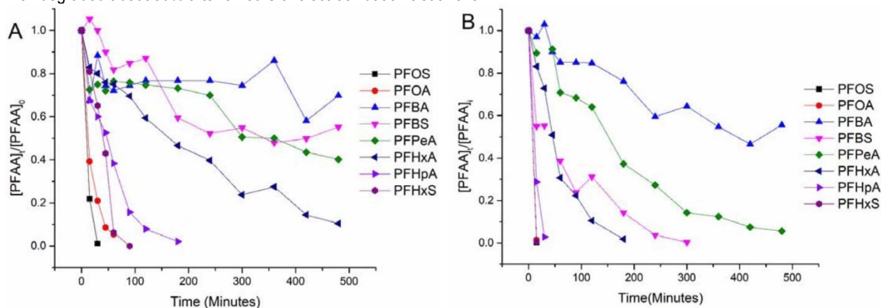
Figure 2 - The concentration of each PFAA over time during electrooxidation with TSO anode at (A) 5 mA/cm 2 and (B) 15 mA/cm 2 . The test solutions contained all PFAAs in a mixture with each at the initial solution of 2.0 μM in 100-mM Na 2 SO 4 as supporting electrolyte.
